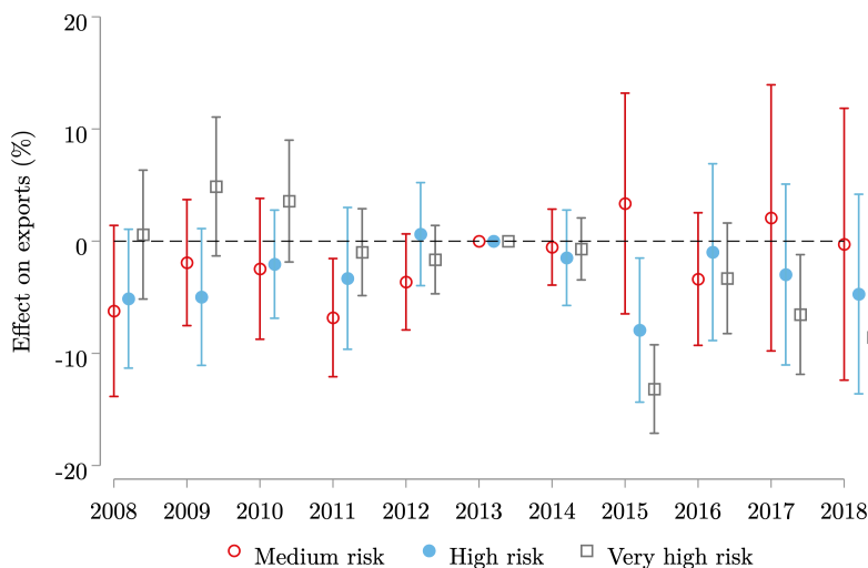
FIGURE C.4: Effect on exports from E.U. countries to high-risk destinations - decomposition across products
